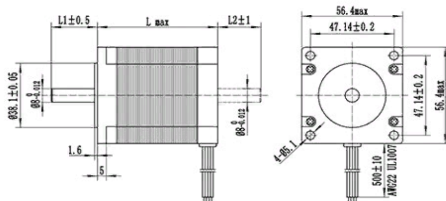
Dimensions unit=mm
